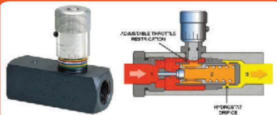
Flow Control Valve
