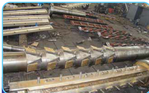
Mandrel Parts
